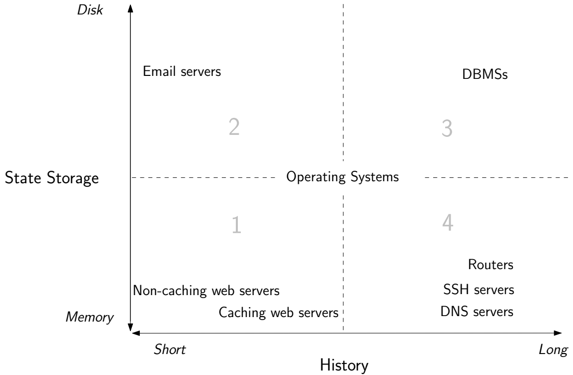
Figure 7.1: Spatio-temporal characteristics of long-running applications.
