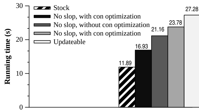
Figure 3.8: KissFFT: impact of optimizations on running time.
