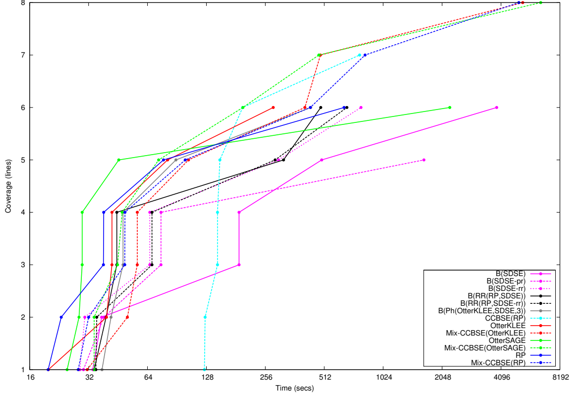
Figure A.28: tac (51 targets). All the strategies did not good very good coverage. But comparing among themselves, Mix-CCBSE strategies performed better, while the SDSE strategies had average performance. We observe that, all the undirected strategies (OtterKLEE, OtterSAGE and random-path) performed better than their Mix-CCBSE versions in the beginning, however these undirected strategies did not make further progress, while the Mix-CCBSE strategies gradually made progress and finally achieved good coverage.
