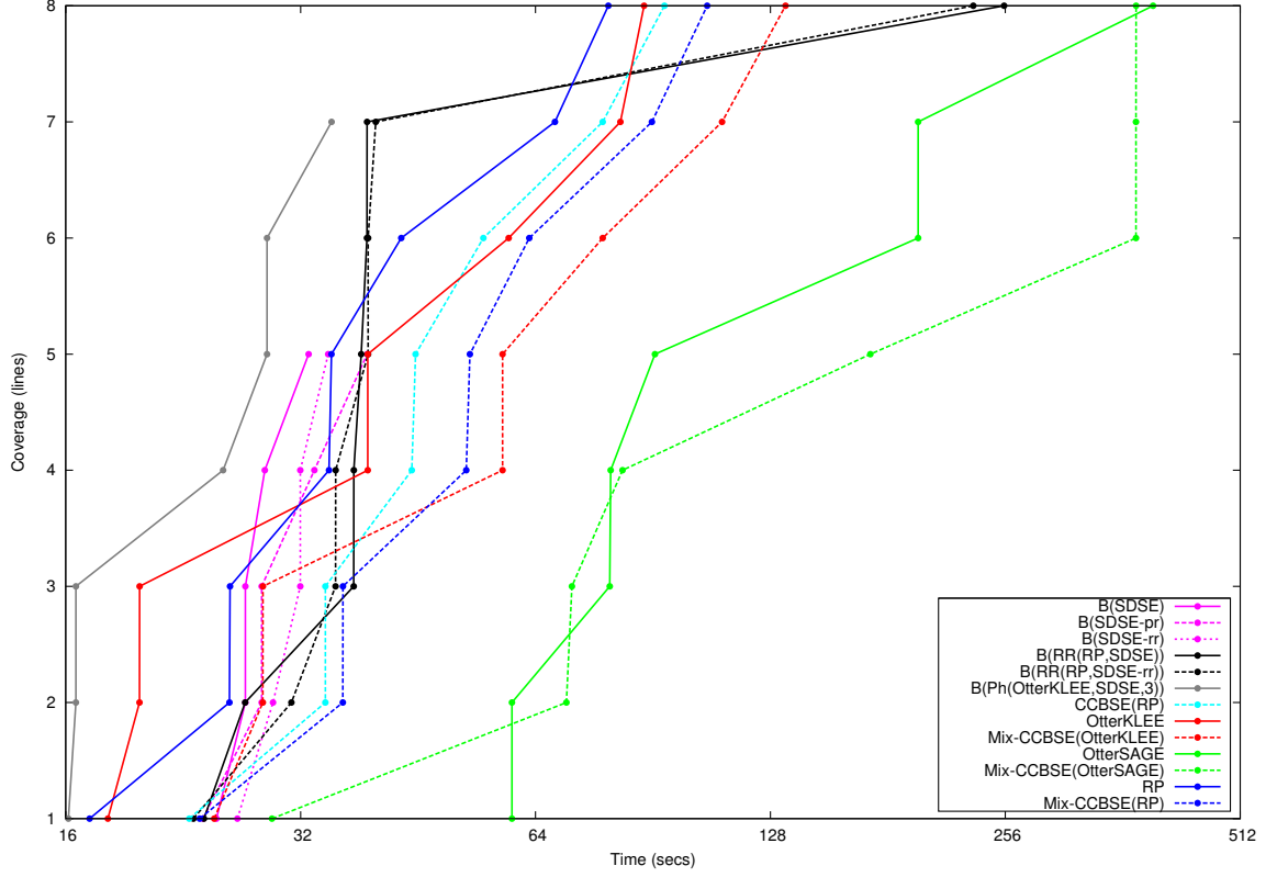
Figure A.20: mkdir (8 targets). Many strategies achieved the full coverage. RP and OtterKLEE reached the full coverage first, while CCBSE(RP), Mix-CCBSE(RP) and Mix-CCBSE(OtterKLEE) achieved the same coverage slightly slower. B(RR(RP,SDSE)), B(RR(RP,SDSE-rr)), OtterSAGE and Mix-CCBSE(OtterSAGE) were able to achieve the same coverage within reasonable time. Notice, however, that B(Ph(OtterKLEE,SDSE,3)) found the first 7 targets much earlier than other strategies (including OtterKLEE).
