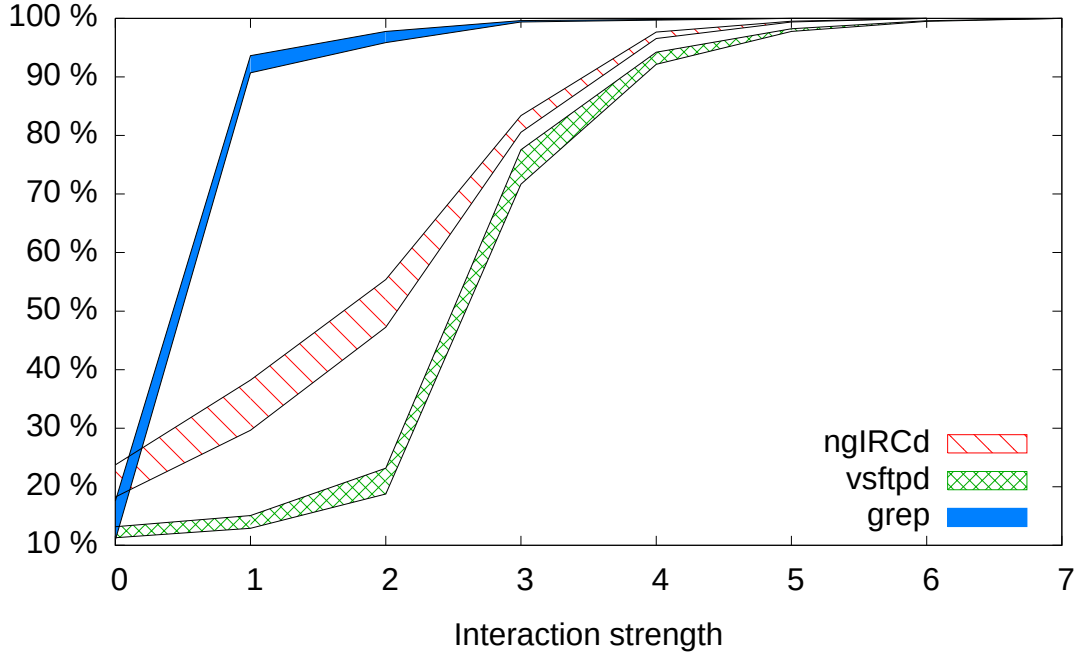
Figure 4.5: Guaranteed coverage versus interaction strength.
