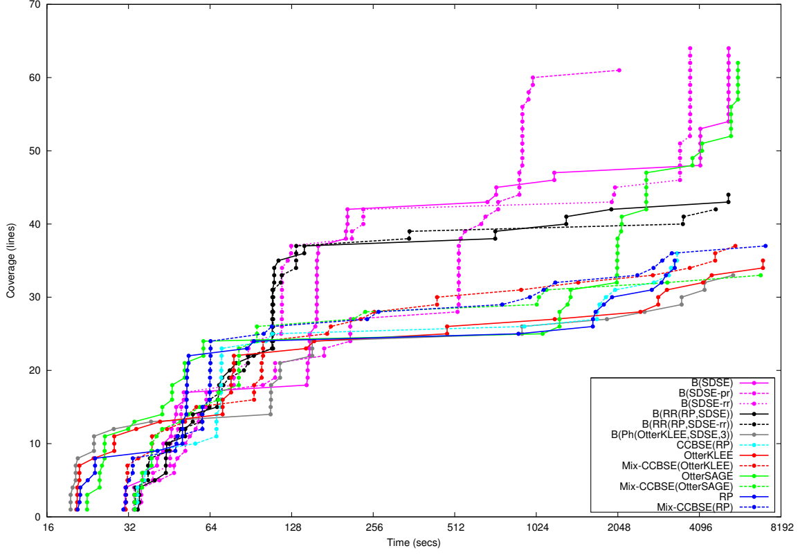
Figure A.25: pr (92 targets). We observe that SDSE strategies dominated others. While they were slow in the beginning, B(SDSE) and B(SDSE-rr) caught up quickly and achieved the highest coverage in the end. B(RR(RP,SDSE)) and B(RR(RP,SDSE-rr)) performed far worse, showing that random-path affects SDSEs and ruins their effectiveness.
